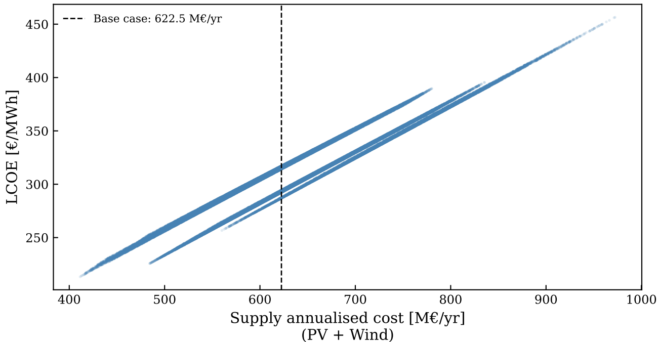
LCOE vs Supply annualised cost
